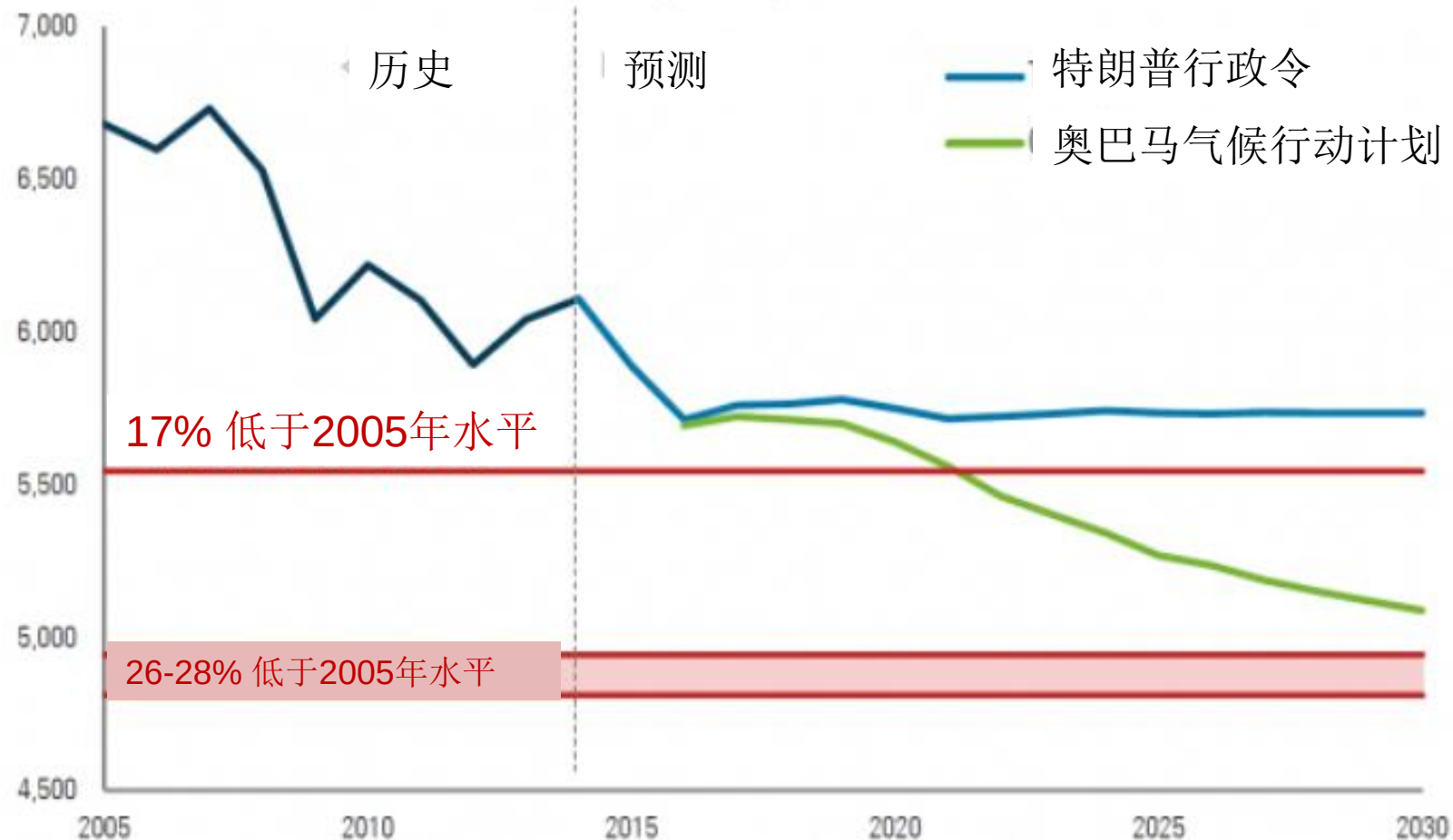
Figure I: US GHG emissions under Trump's Executive Order and Obama's Climate Action Plan
