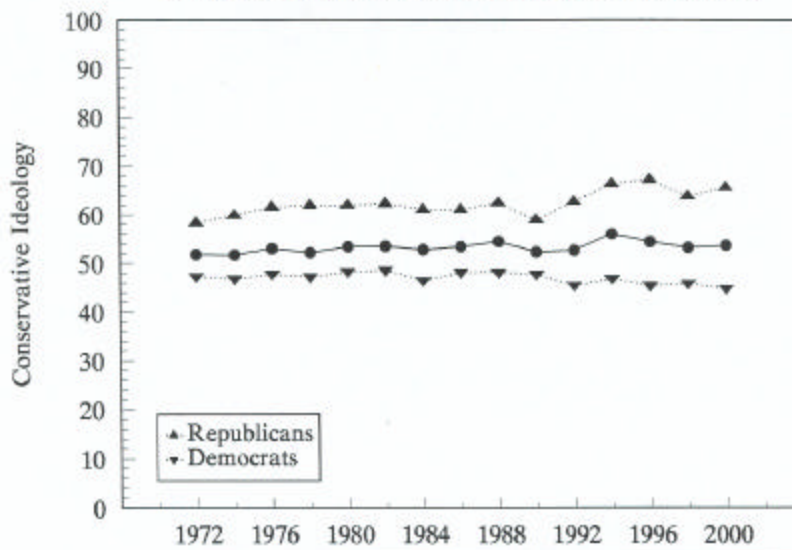
Liberal-Conservative Ideology, 1972-2000
