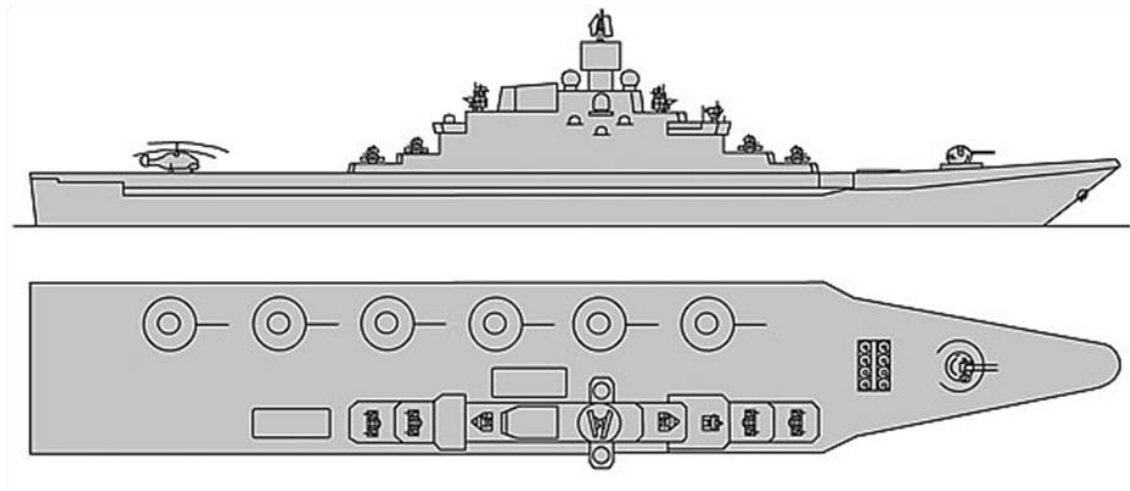
Figure 5. Line drawing of Project 11780 71
