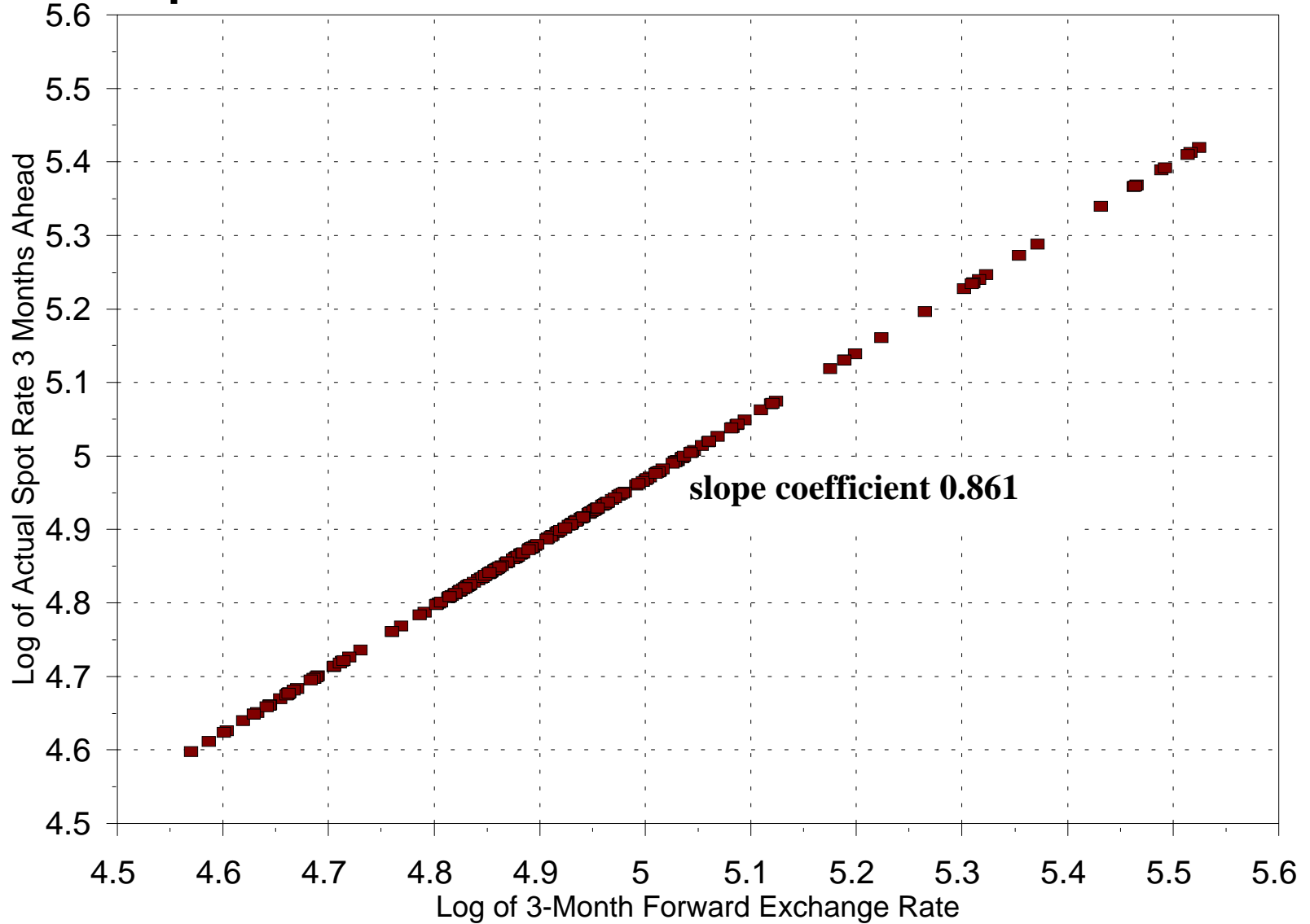
Figure 18 -- Regression Line
